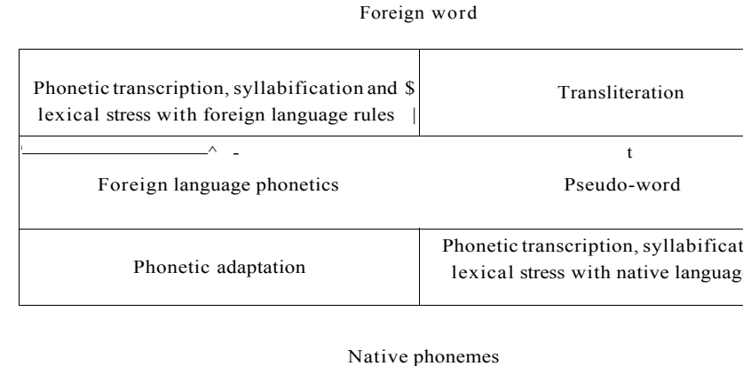
Figure 2: Foreign word handling in TTS synthesis
