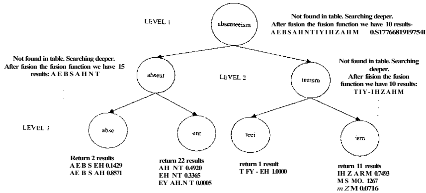
Figure 1: Execution of DLOPS for the word "absenteeism"
