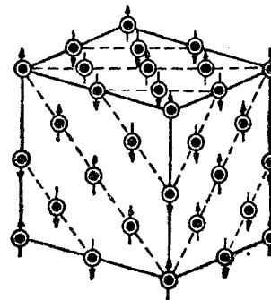
Antiferomagnetic
