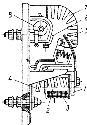
Contactor
