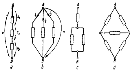
Circuit electric a — serie; b — paralel; c — serie-paralel; d — complex
