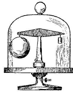
Baroscop
