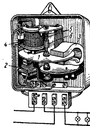
Contor monofazat
