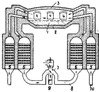
Cuptor Siemens-Martin
