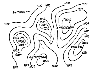
Sistem baric
