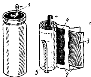
Condensator electrolitic
