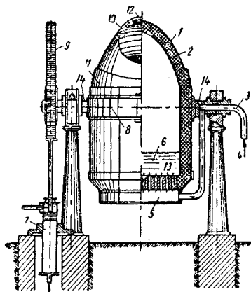
Convertizor
